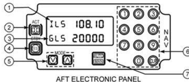
AFT ELECTRONIC PANEL
